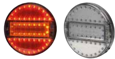
Part No. 800733 TAIL LIGHT 3 FUNCTIONS LED
